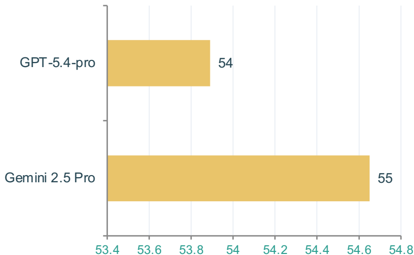
VISTA Vision-Language
