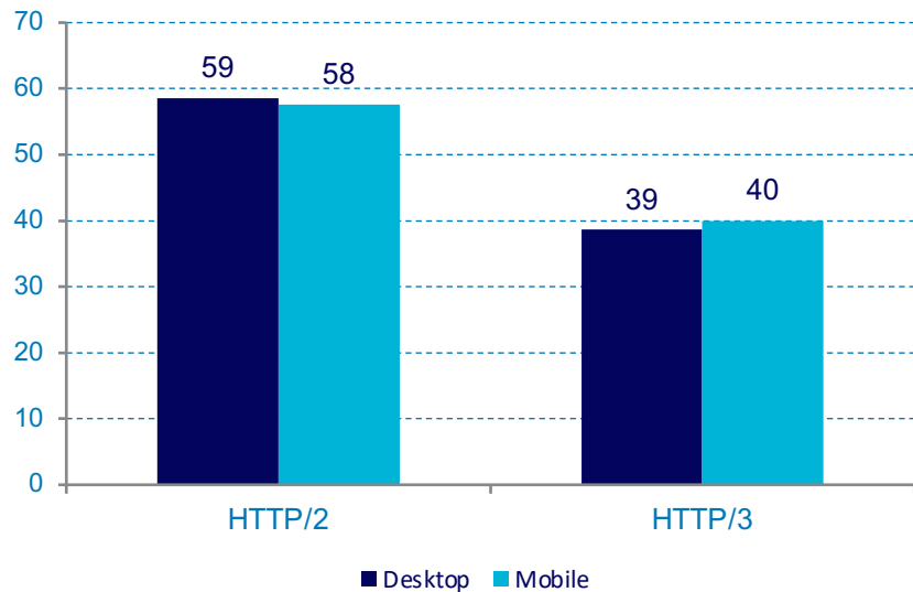
Protocol Adoption (Latest)
