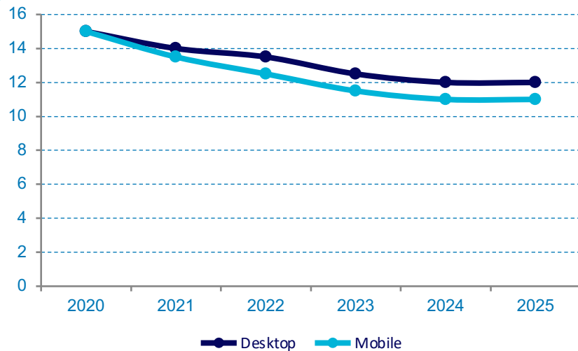
TCP Connections per Page (median)
