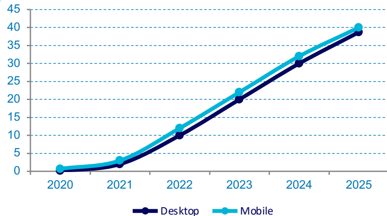
HTTP/3 Support Growth
