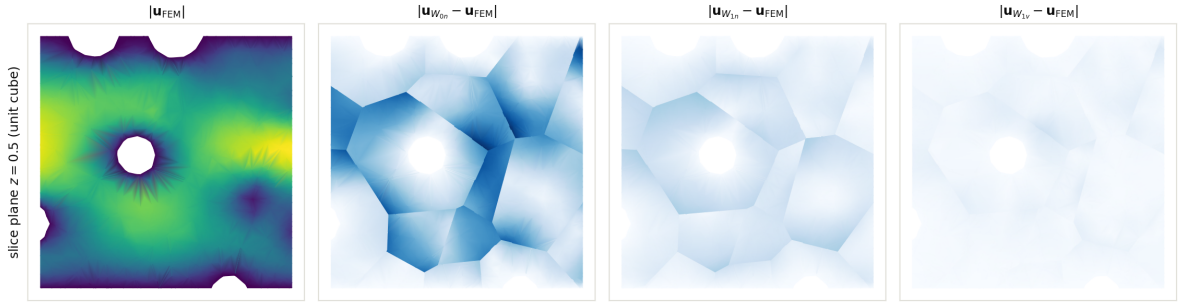
Figure 4: Random-27, slice z = 0.5 : FEM velocity magnitude (left) and pointwise velocity error magnitude of \mathcal{W}_{0n} , \mathcal{W}_{1n} , \mathcal{W}_{1v} on a common color scale (blue = zero error). Error maps share one scale; the reference panel has its own.
