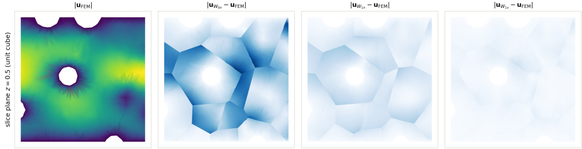
Figure 4: Random-27, slice z = 0.5 : FEM velocity magnitude (left) and pointwise velocity-error magnitude of \mathcal{W}_{0n} , \mathcal{W}_{1n} and \mathcal{W}_{1v} with a common archived color normalization. The panel is qualitative because numerical colorbar limits were not retained in the archived image.
