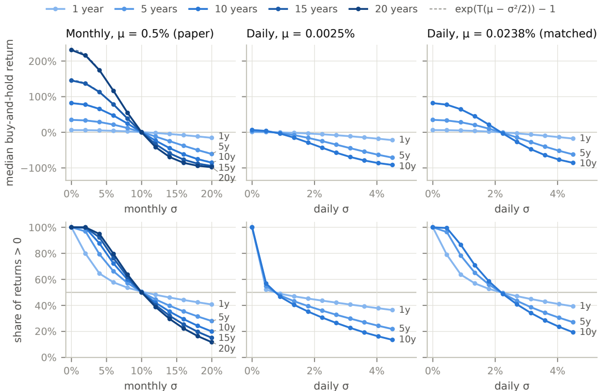
Figure 1: Median buy-and-hold return (top) and share of positive outcomes (bottom) against volatility, by horizon (seed 0). Dashed lines show the lognormal approximation of the median, e^{T(\mu - \sigma^2/2)} - 1 .
