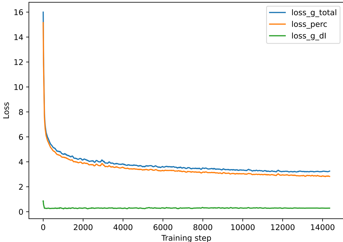
Convergence: Generator losses
