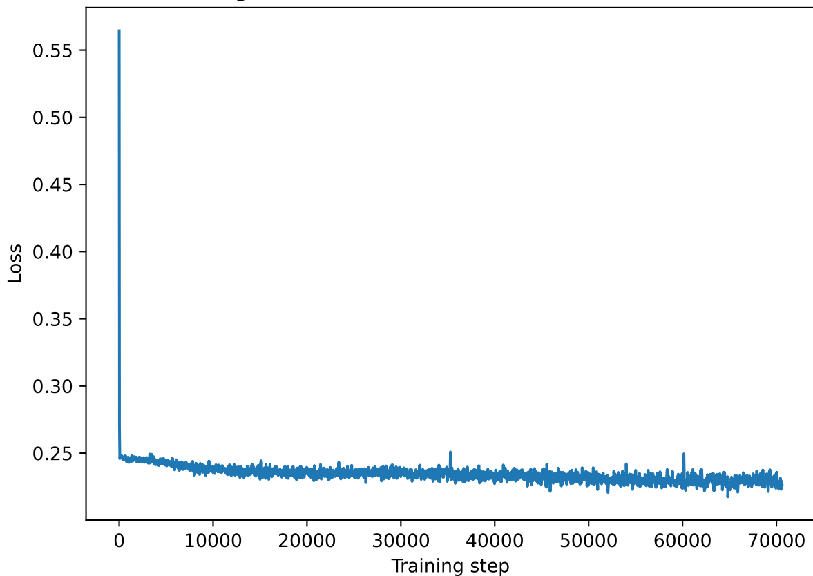
Stage-2 (128×128 mouth): Discriminator loss
