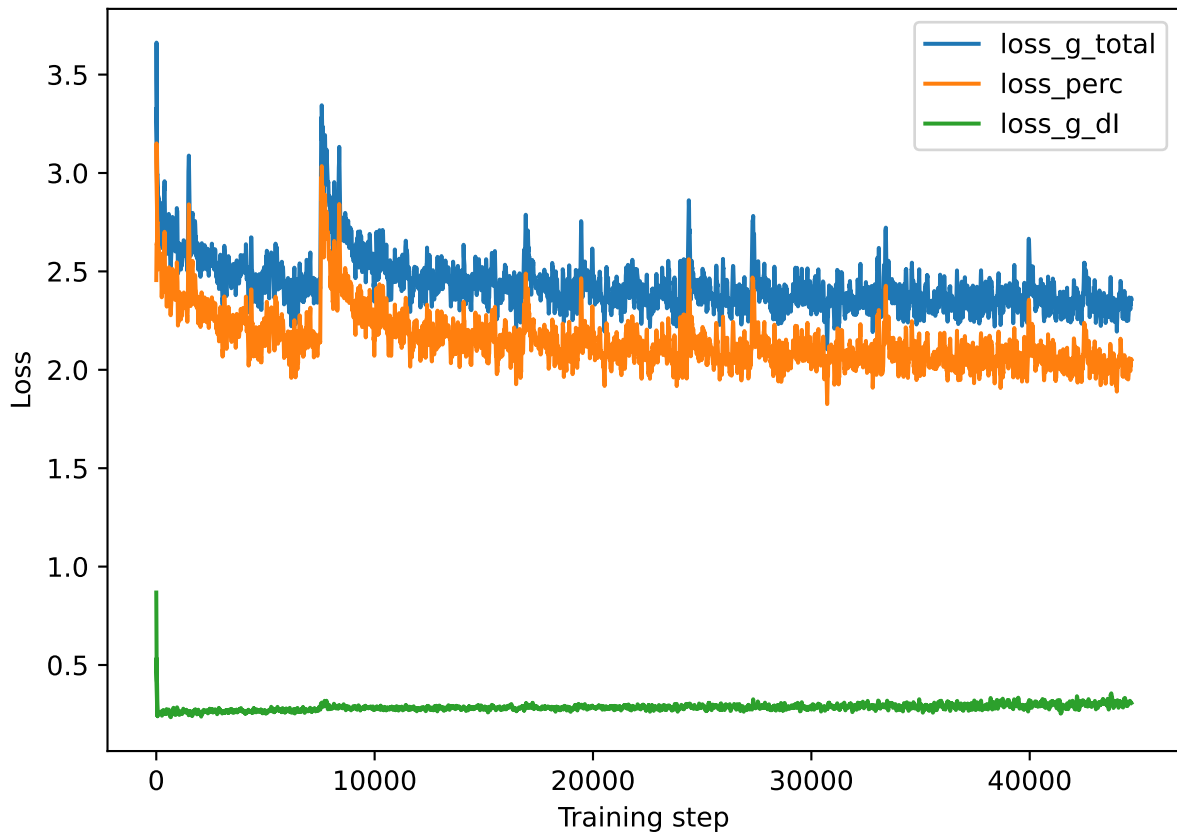
Stage-3 (256×256 mouth, frame): Generator losses
