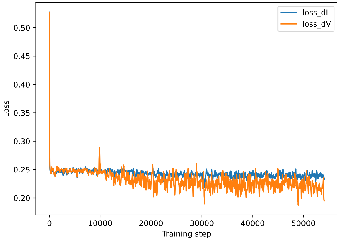
Stage-4 (clip): Discriminator losses
