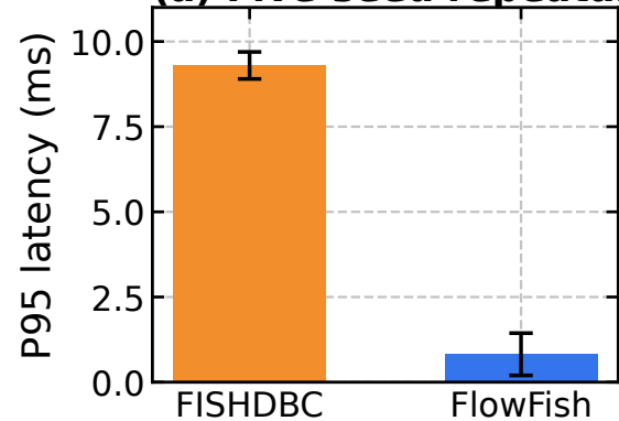
(a) Five-seed repeatability
