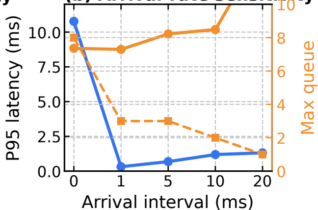
(b) Arrival-rate sensitivity
