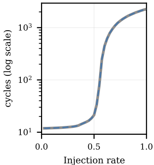
Bit-Reversal: latency
