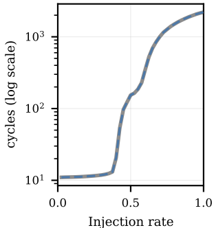
Diagonal-3D: latency
