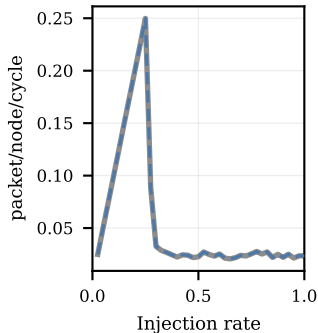
Perfect Shuffle: reception
