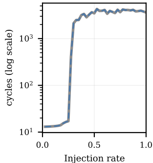
Perfect Shuffle: latency
