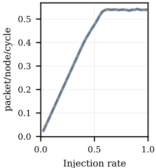
Diagonal-3D: reception
