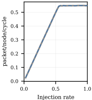
Bit-Reversal: reception
