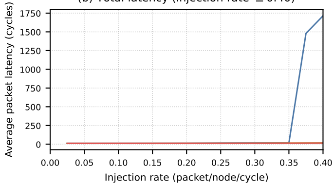
(b) Total latency (injection rate \leq 0.40 )
