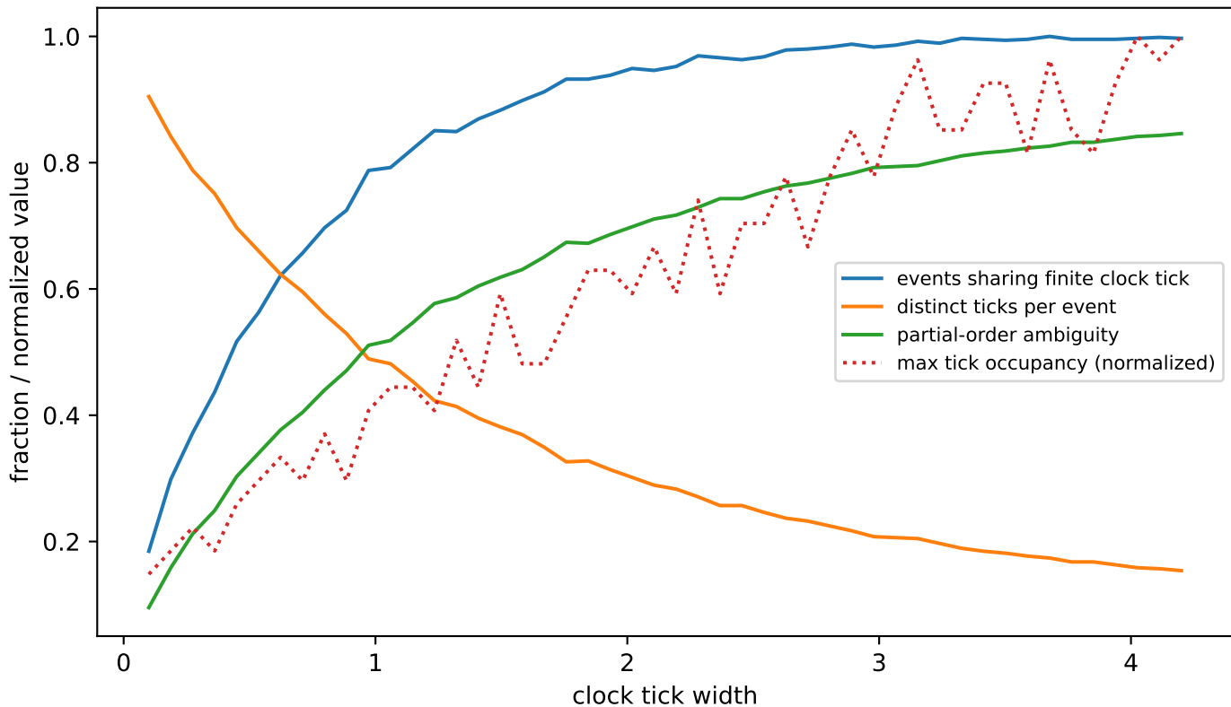
Finite clock precision coarsens temporal order
