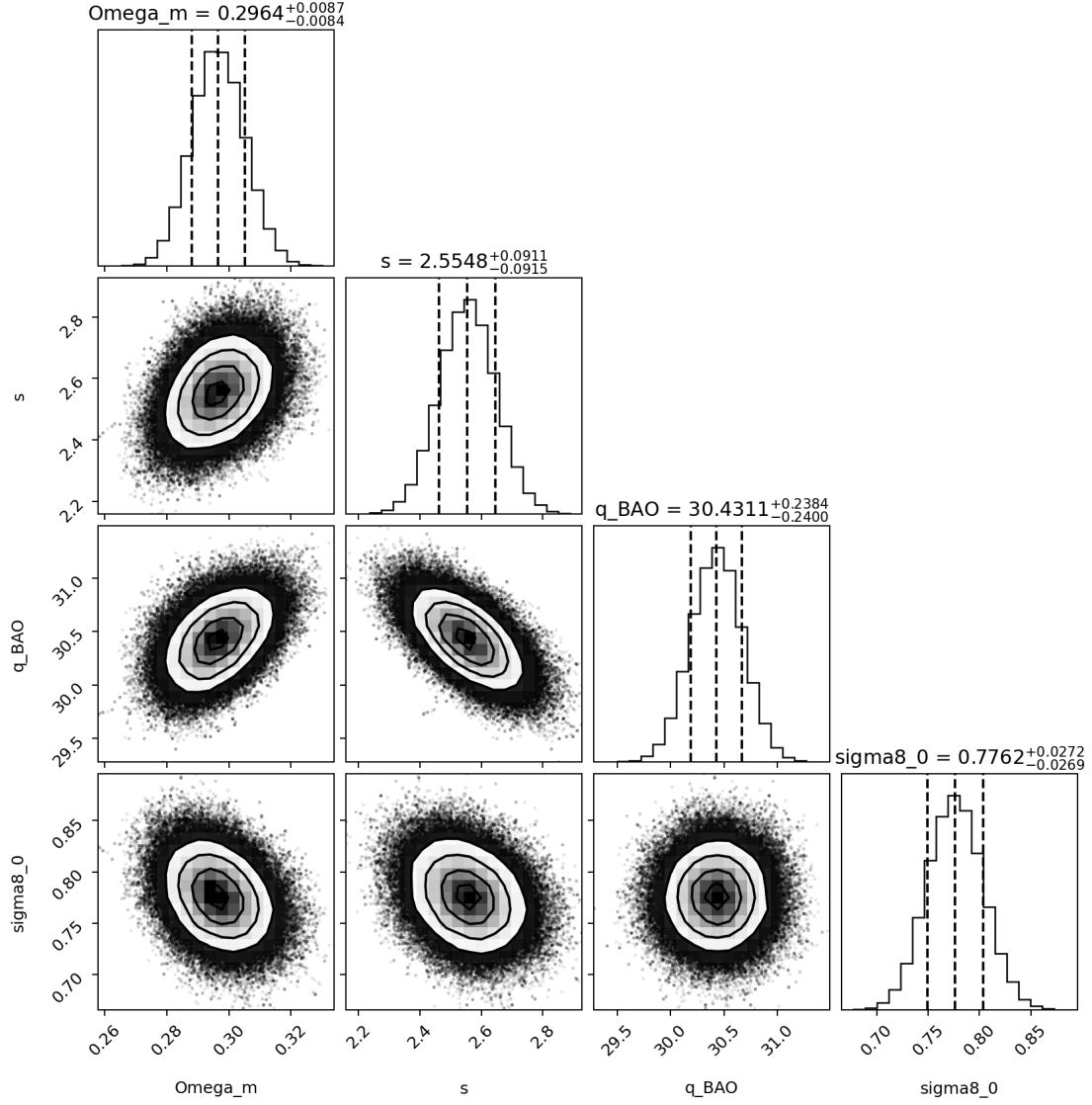
Figure 6: Combined three-seed exact posterior for G1DE- M_{3/4} . The s = 3 value marks the \Lambda CDM-like filling limit. The derived \Sigma_0 = -\frac{3}{4}(3 - s) gives \Sigma_0 < 0 with P(\Sigma_0 < 0) = 1.0 .
