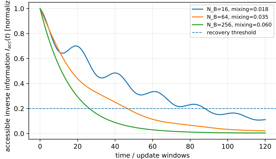
Finite-bath memory decay with finite recurrence
