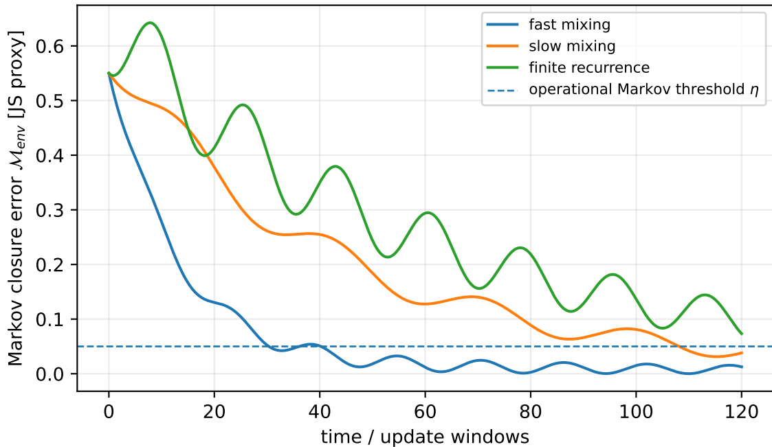
Markovianization as loss of accessible bath memory
