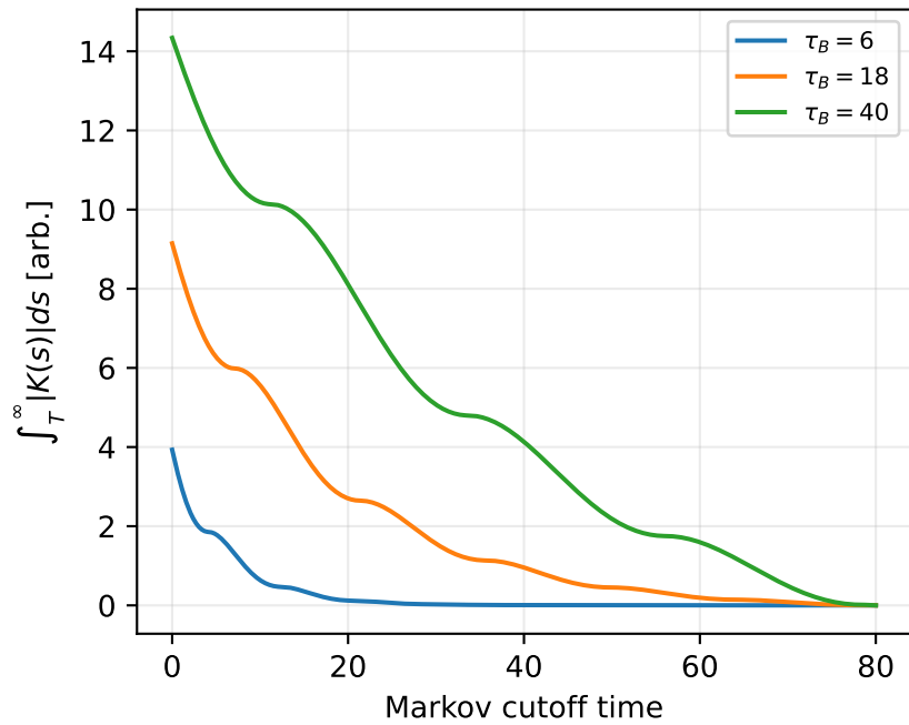
Unresolved memory tail burden
