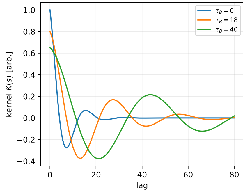
Finite-bath memory kernels
