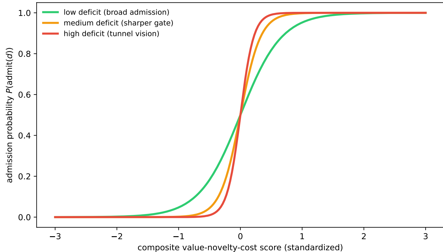
Synthetic normal-form illustration: sigmoid admission curves and tunnel vision
