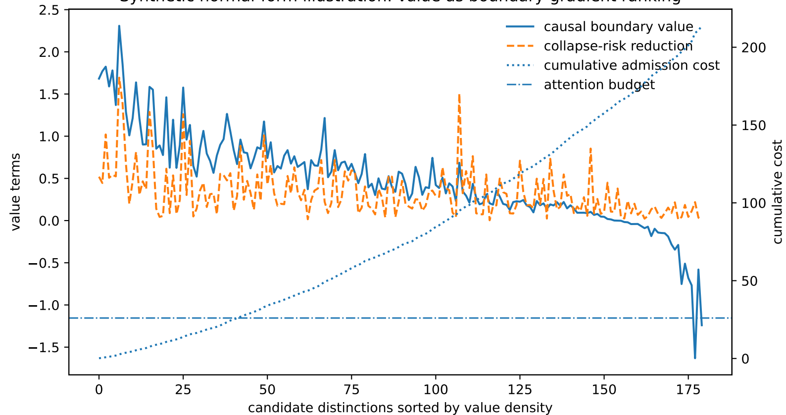
Synthetic normal-form illustration: value as boundary-gradient ranking
