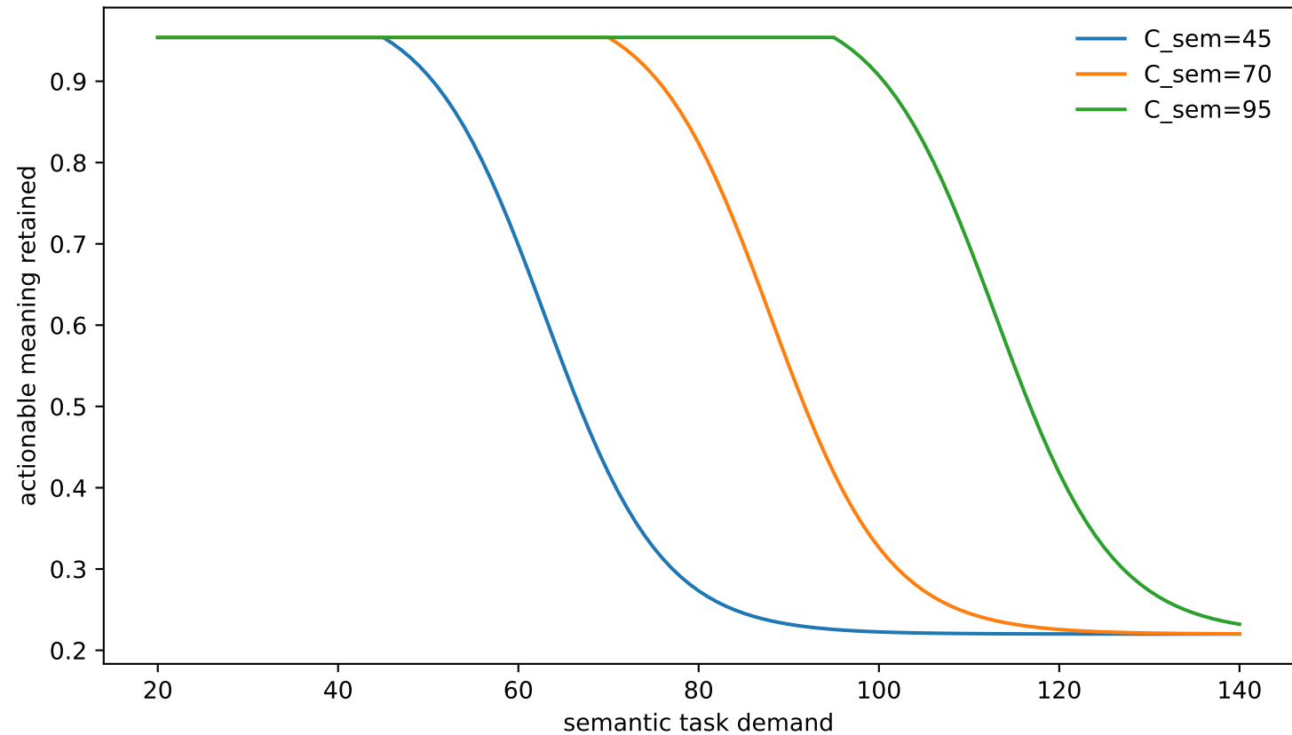
Synthetic normal-form illustration: semantic capacity deficit and collapse
