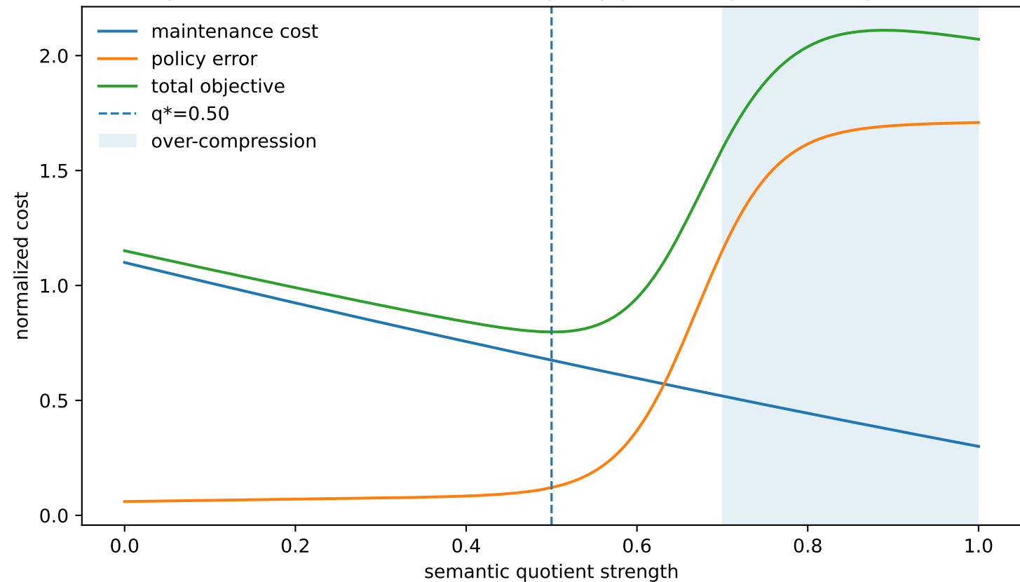
Synthetic normal-form illustration: policy-preserving semantic quotient
