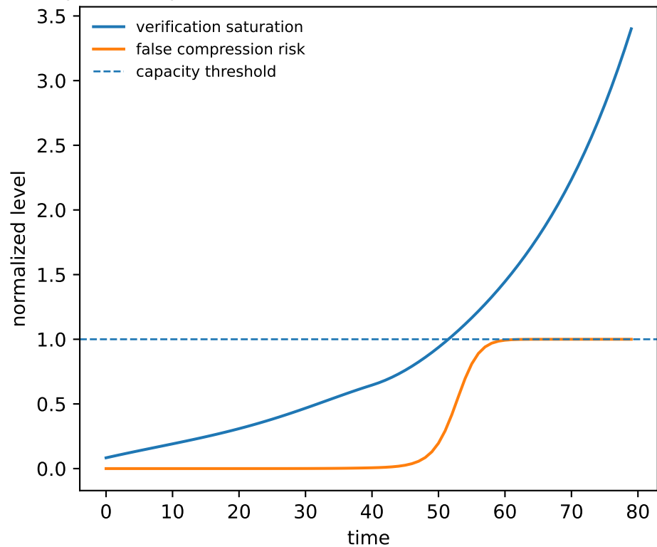
Epistemic pollution as verification bandwidth saturation
