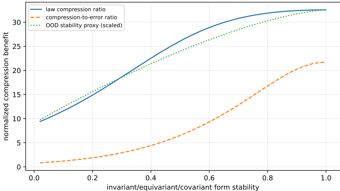
Invariant-form stability improves law compression
