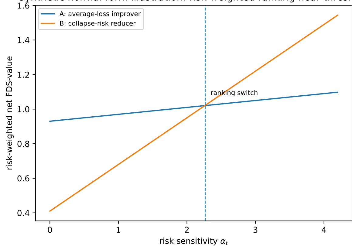
Synthetic normal-form illustration: risk-weighted ranking near threshold
