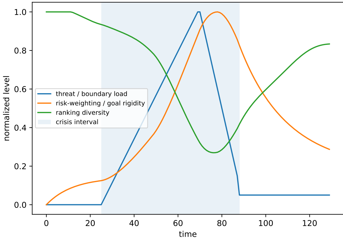
Synthetic normal-form illustration: goal hysteresis and recovery lag
