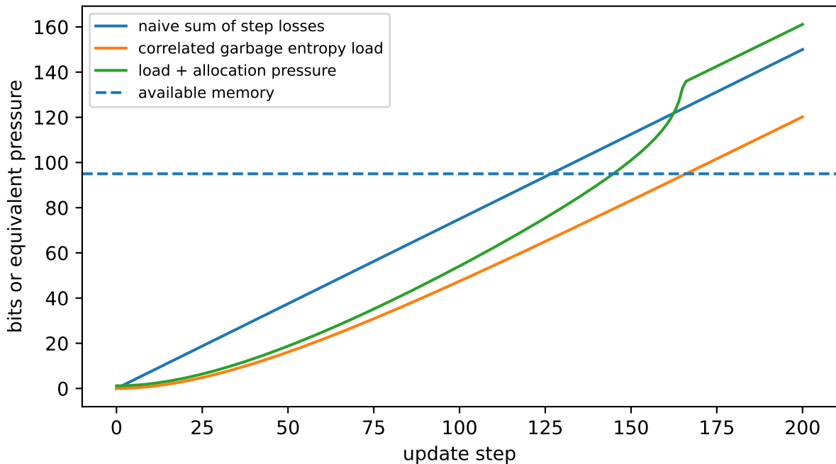
Correlated garbage and nonlinear memory-fill pressure
