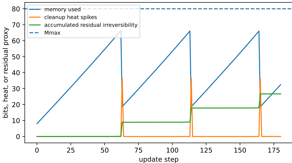
Finite memory turns delayed erasure into cleanup events
