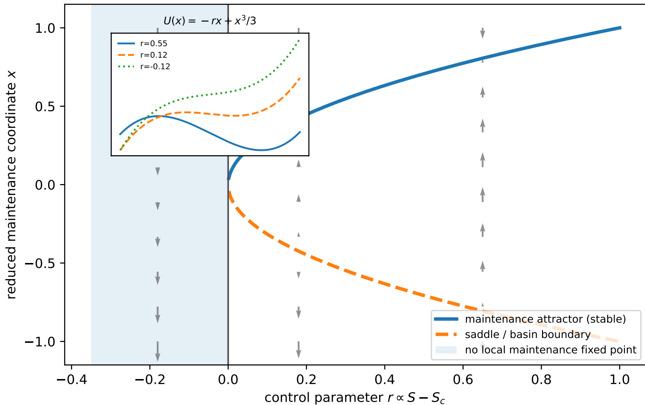
Reduced saddle-node structure of maintenance-attractor loss
