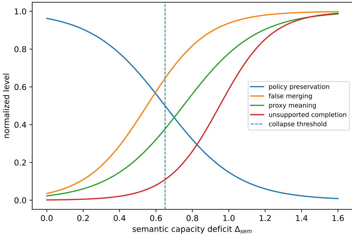
Synthetic normal-form illustration: semantic deficit and collapse
