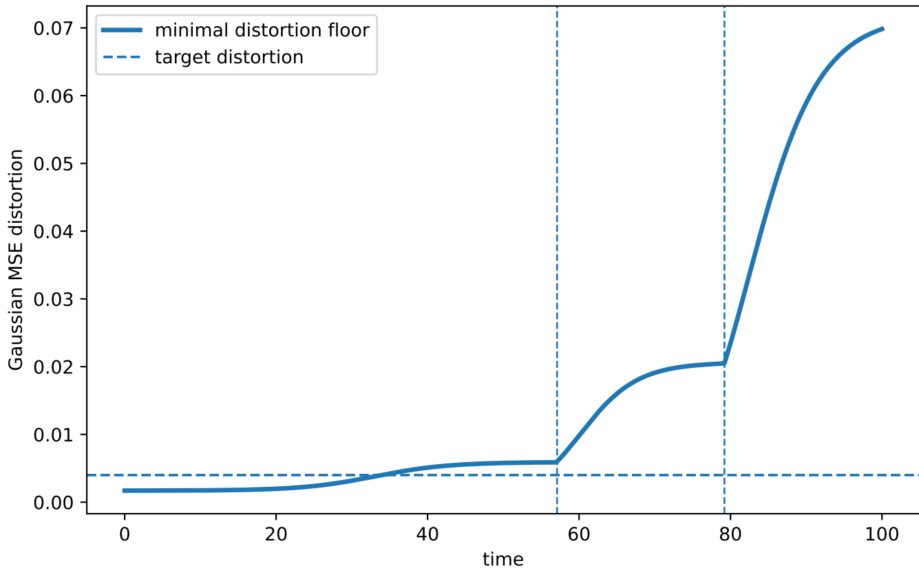
Rate-distortion error floor under bottleneck collapse
