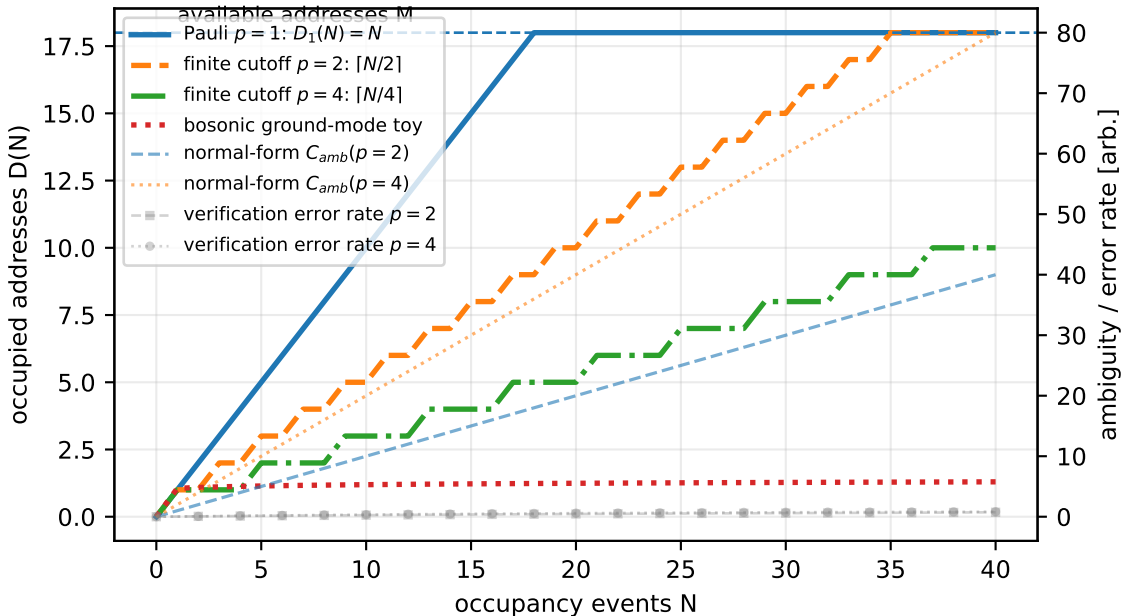
Address diversity and multi-occupancy ambiguity cost
