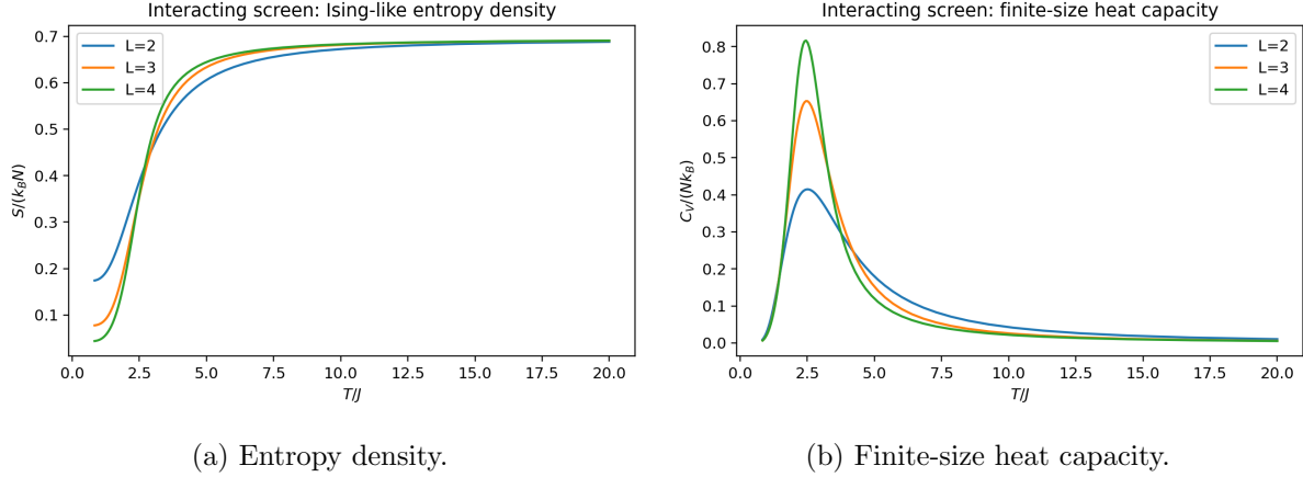
Figure 4: Exact enumeration of small Ising-like interacting screens.
