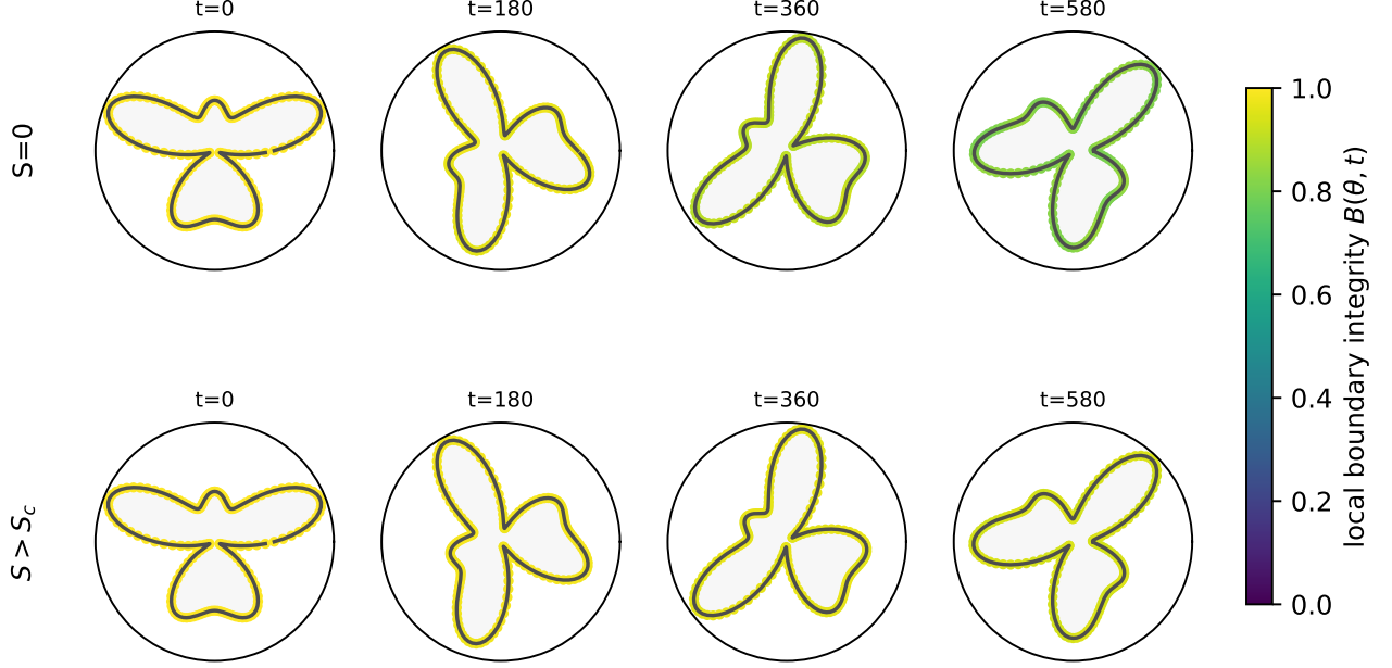
FIG. 4. Spatial failure mode II: phase-field-inspired reduced dynamic-boundary failure. Grey outlines show the boundary radius field R(\theta, t) ; color along the boundary shows local integrity B(\theta, t) . The dominant failure signal is not necessarily gross shape change but loss of local integrity. Thus similar outlines can correspond to very different leakage or damage states. The model uses a reduced radius/integrity field rather than a full Cahn-Hilliard, Allen-Cahn, Helfrich, or hydrodynamic membrane solver.
