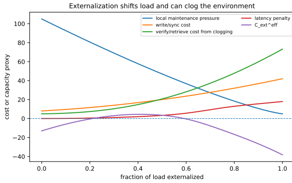
FIG. 4. Externalization shifts load and can clog the environment. Local maintenance pressure falls as more records are externalized, but write, verification, retrieval, and latency costs grow. Effective external capacity can become negative when environmental record load increases.
