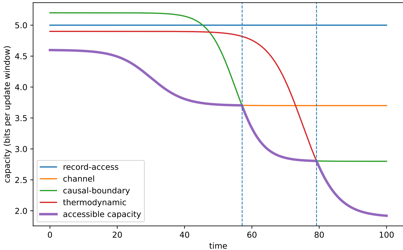
Finite-observer accessible capacity as a bottleneck minimum
