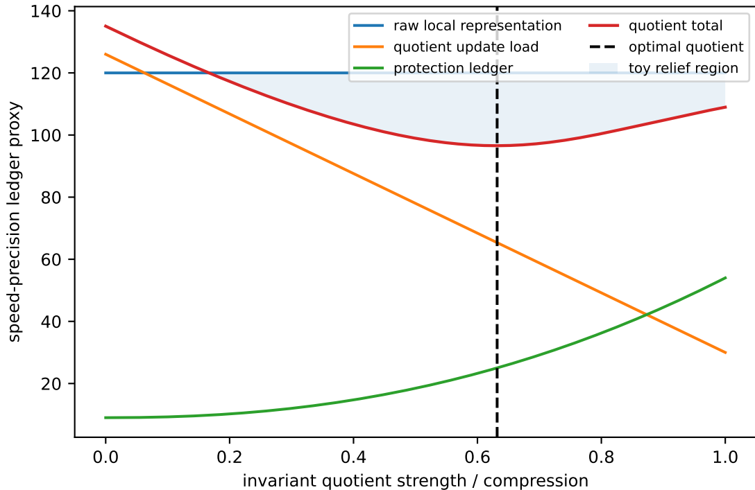
Invariant compression can reduce maintenance burden
