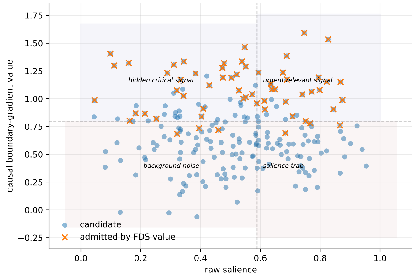
Synthetic normal-form illustration: salience-value dissociation
