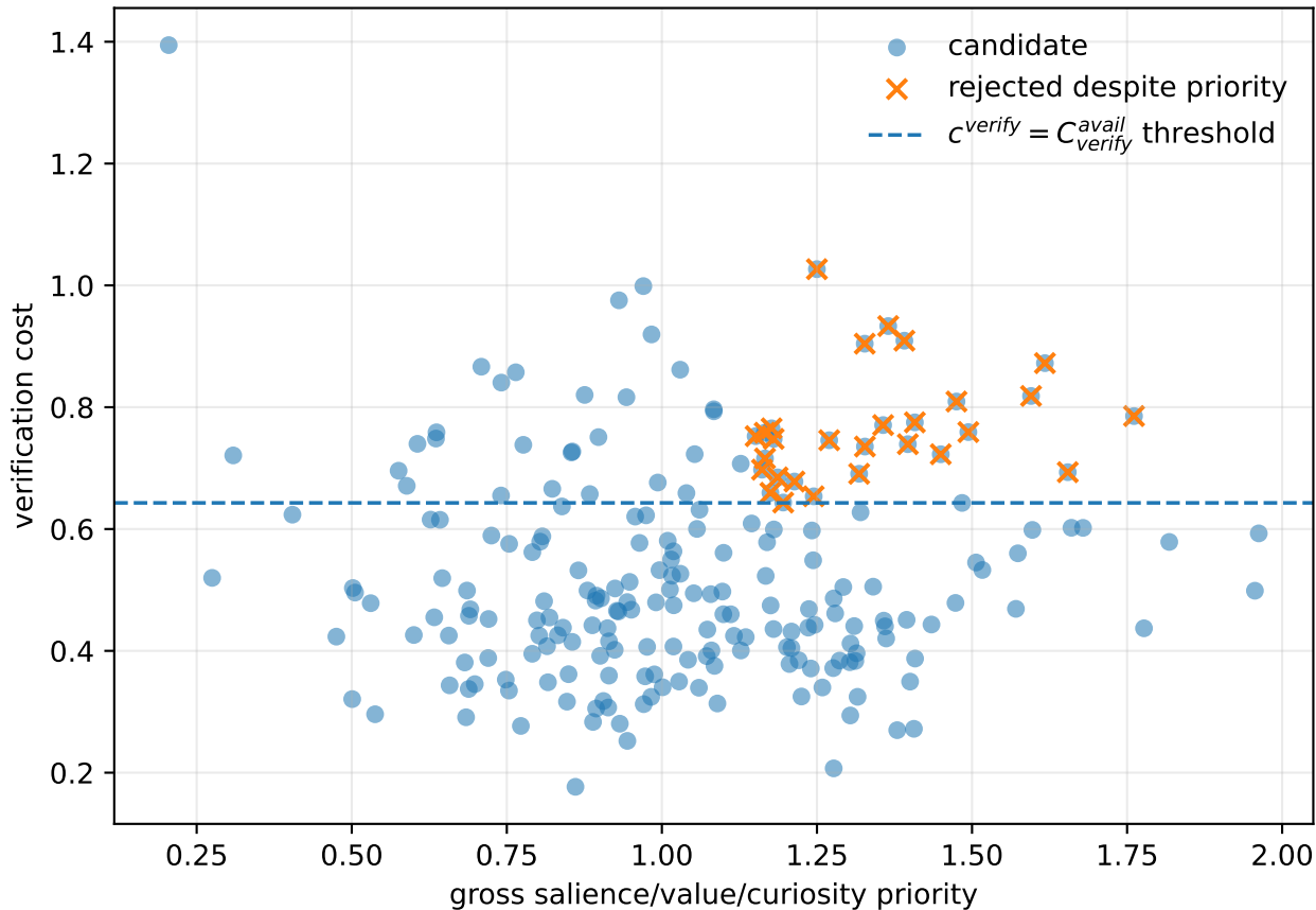
Synthetic normal-form illustration: verification-limited attention
