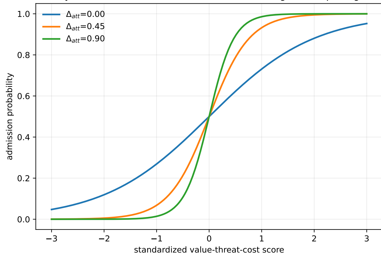
Synthetic normal-form illustration: nonlinear gate steepening
