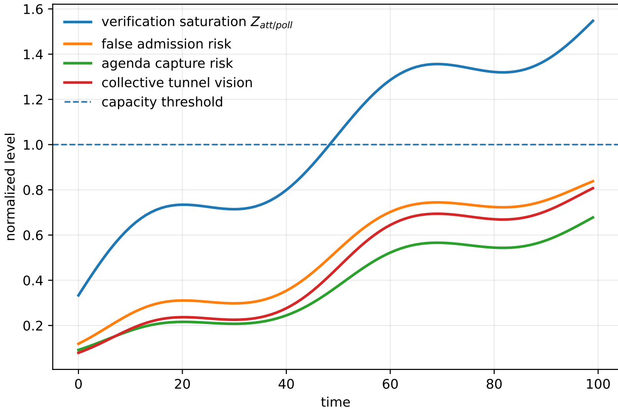
Synthetic normal-form illustration: collective attention and epistemic pollution
