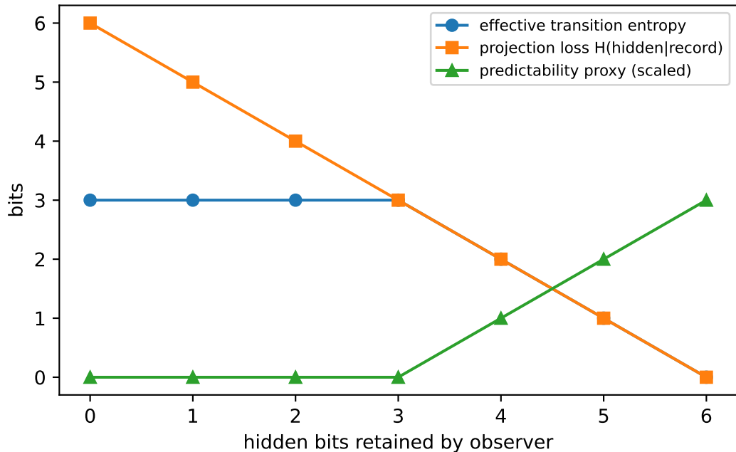
Projection-induced stochasticity falls as hidden distinctions are retained
