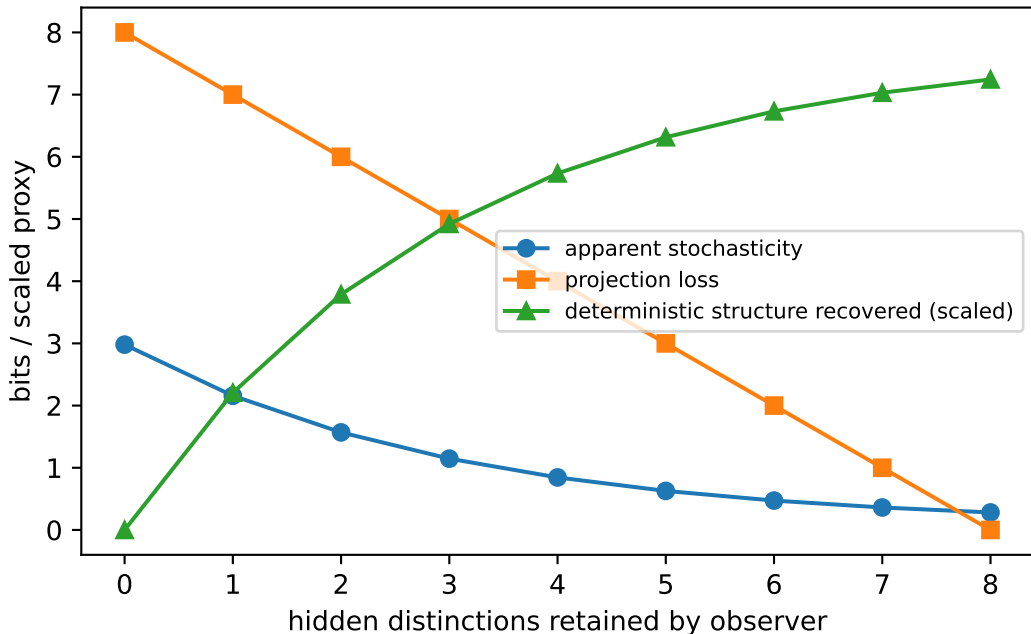
Randomness can shrink as observer capacity increases
