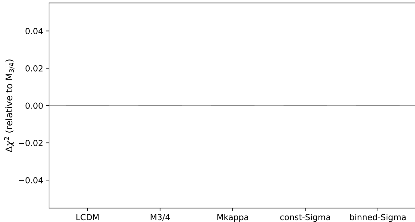
KiDS-1000 shear-only: M_{3/4} vs controls ( m_i + \Delta z_i + A_{IA} profiled)
