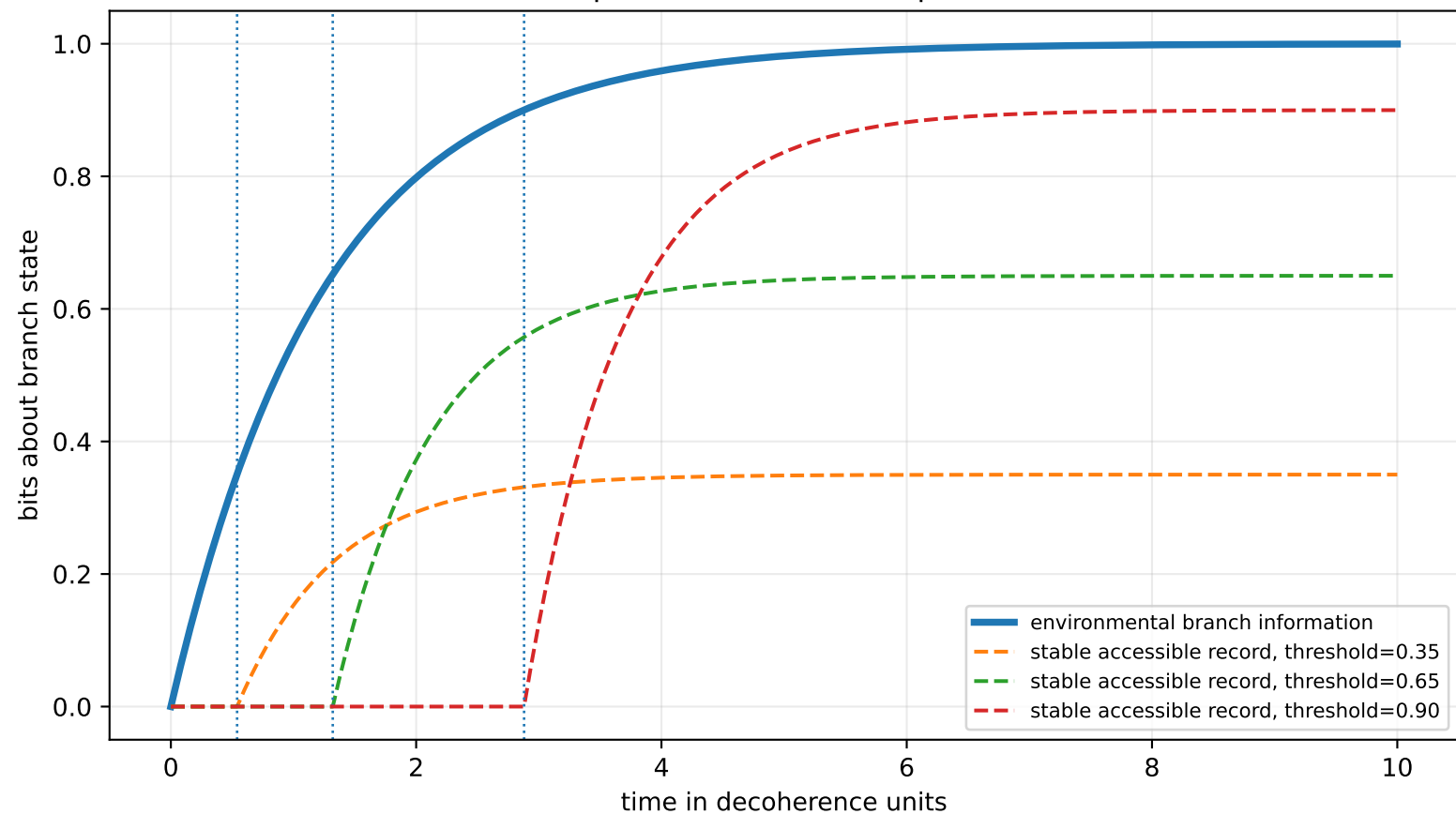
Interface with decoherence: operational records require finite accessible stabilization
