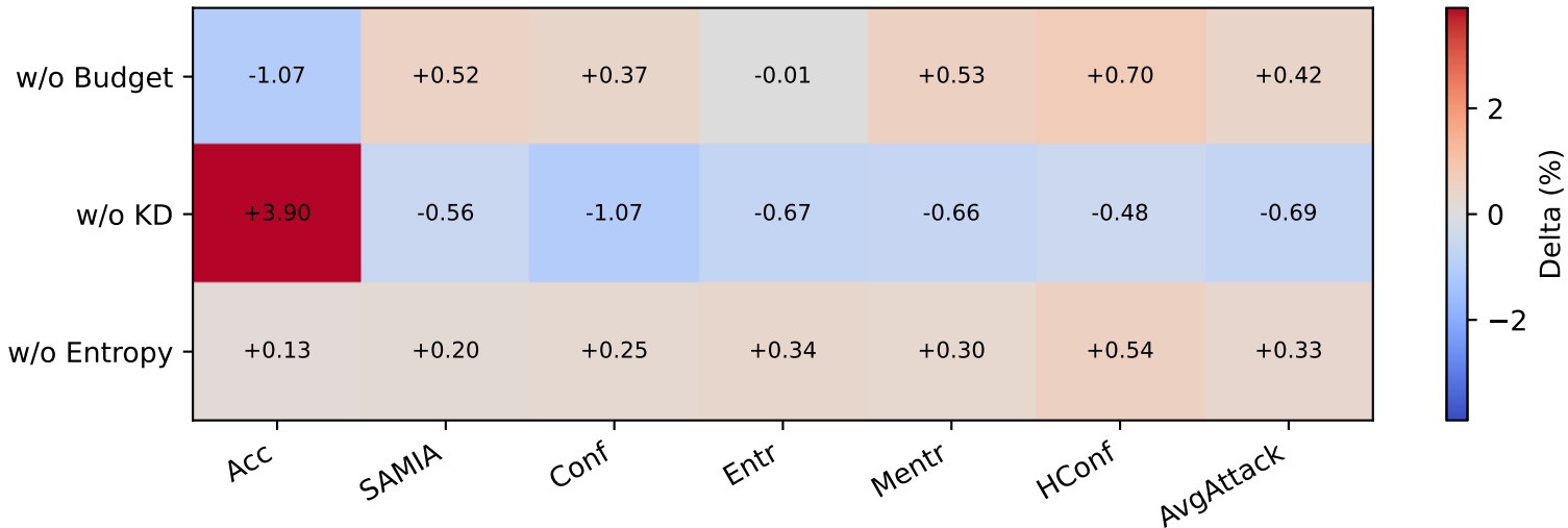
CIFAR100 Ablation Delta vs Full
