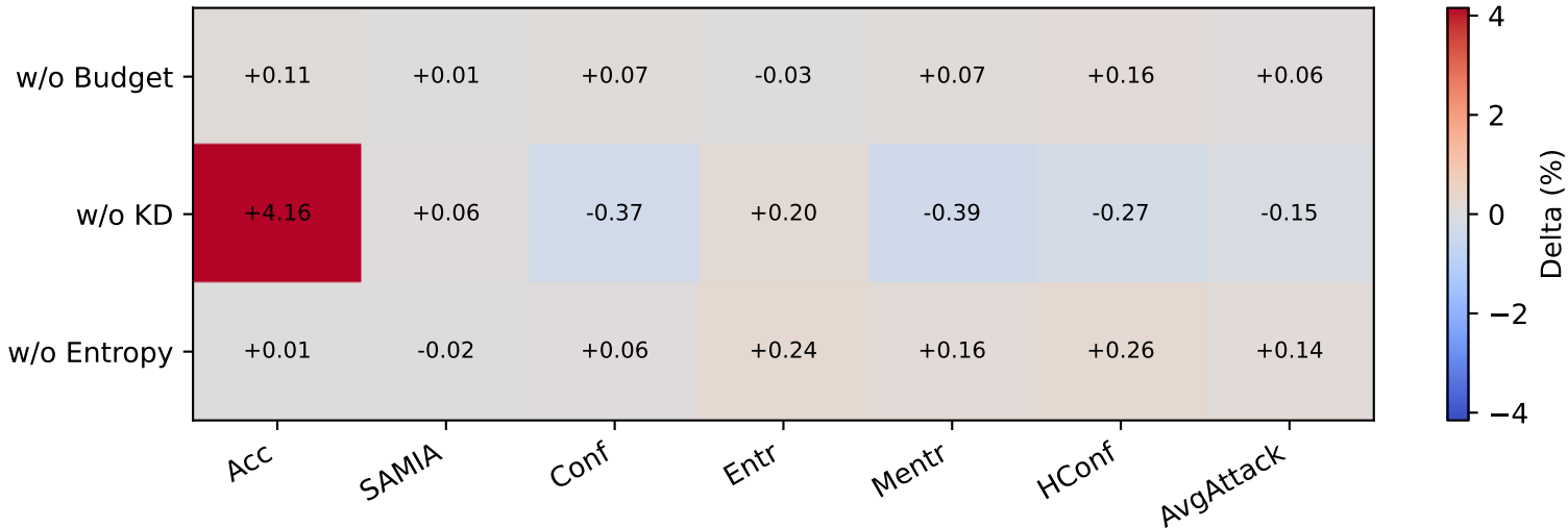
CINIC Ablation Delta vs Full
