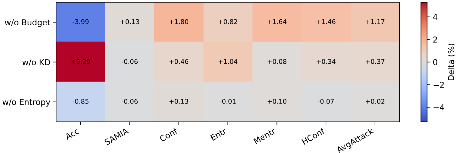
RESISC45 Ablation Delta vs Full
