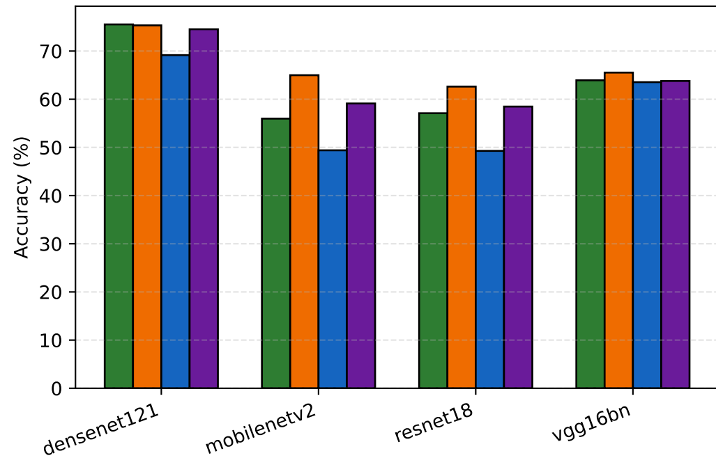
Victim Pruned Accuracy
