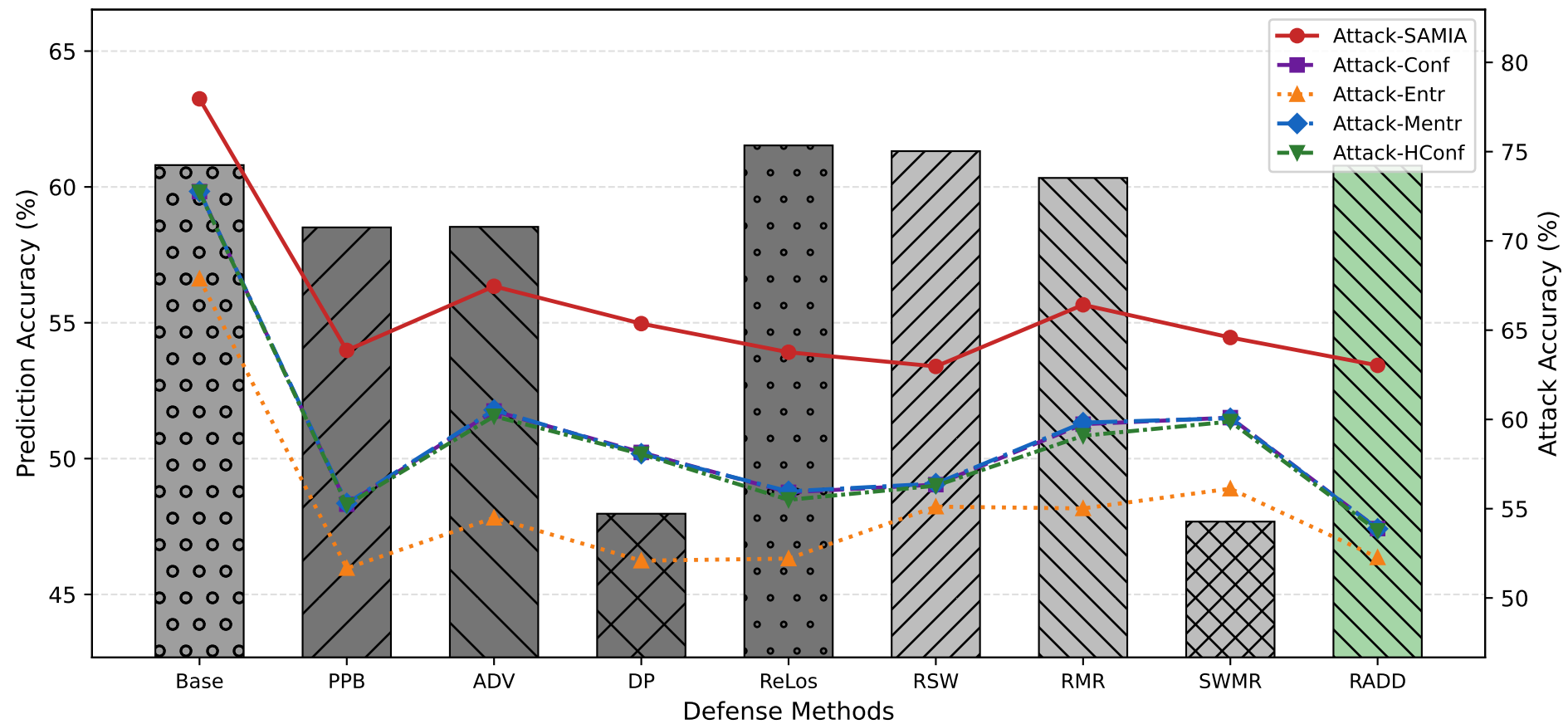
(Cinic Resnet18)
