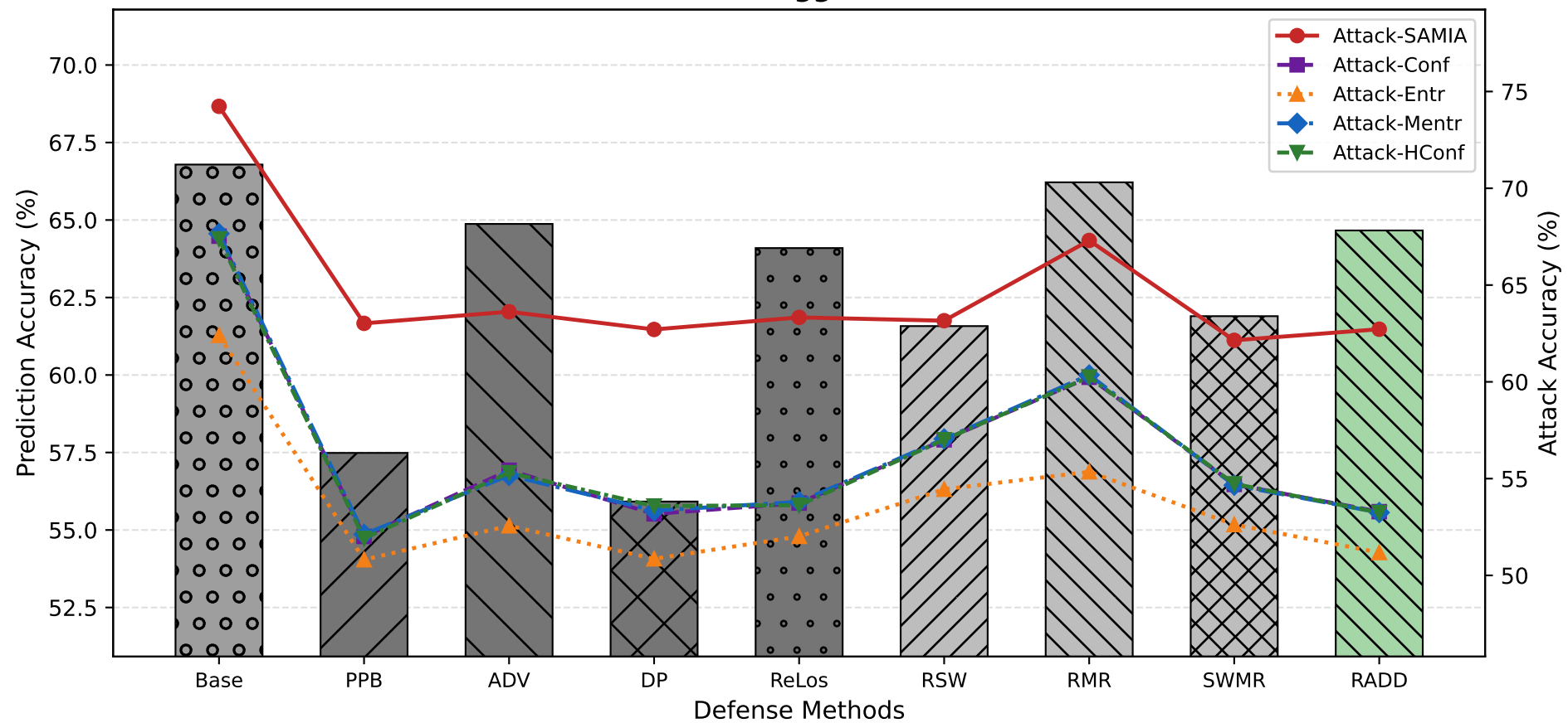
(Cinic Vgg16bn)
