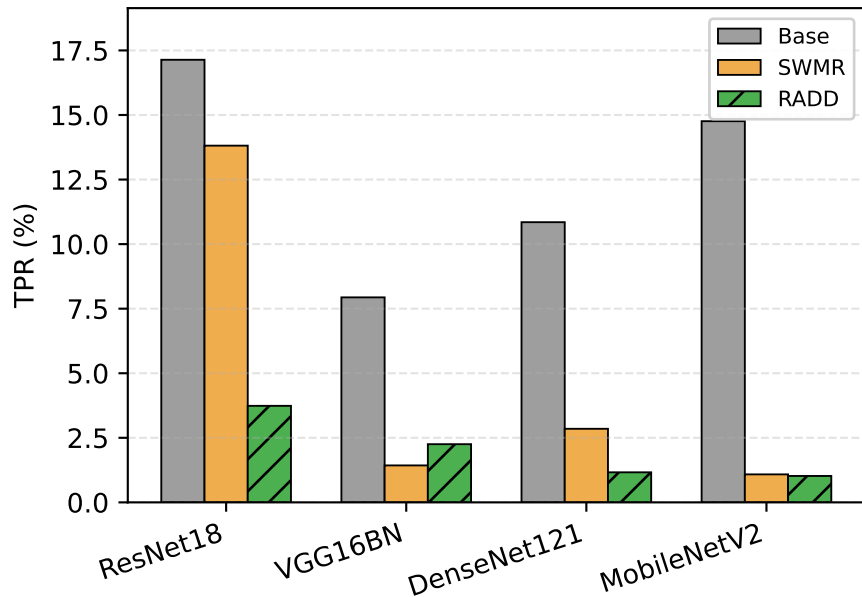
LiRA TPR@0.5%FPR
